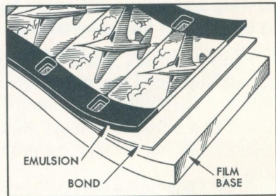
Diagram showing construction of movie films.
